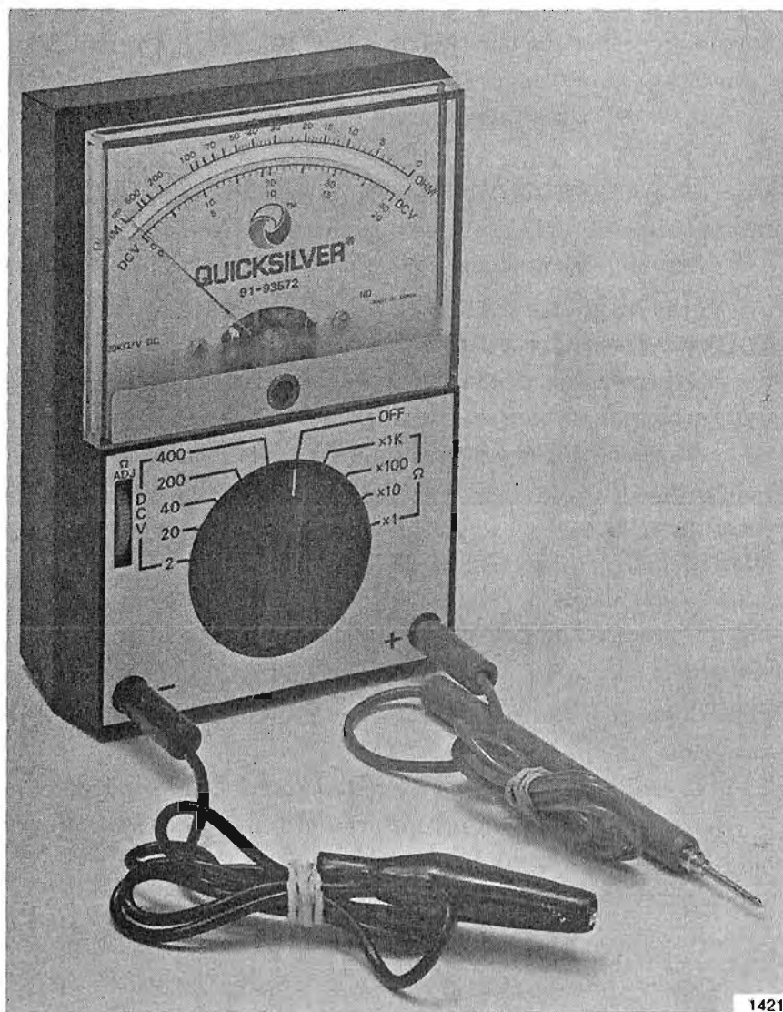
Figure 2. Quicksilver Volt/Ohm Meter (91-93572)
