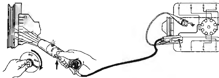
Figure 1. Portable Timing Light
