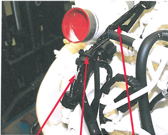
Original wire to turbo cable strap 06V 971 130 Adaptor Harness
